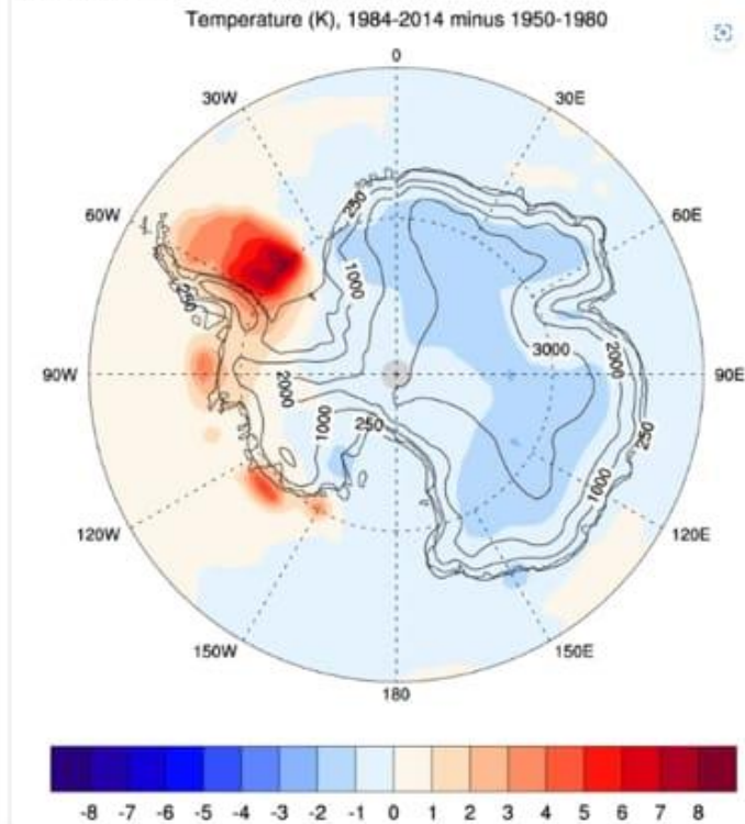
Fig. 1: Observed surface temperature anomaly.
